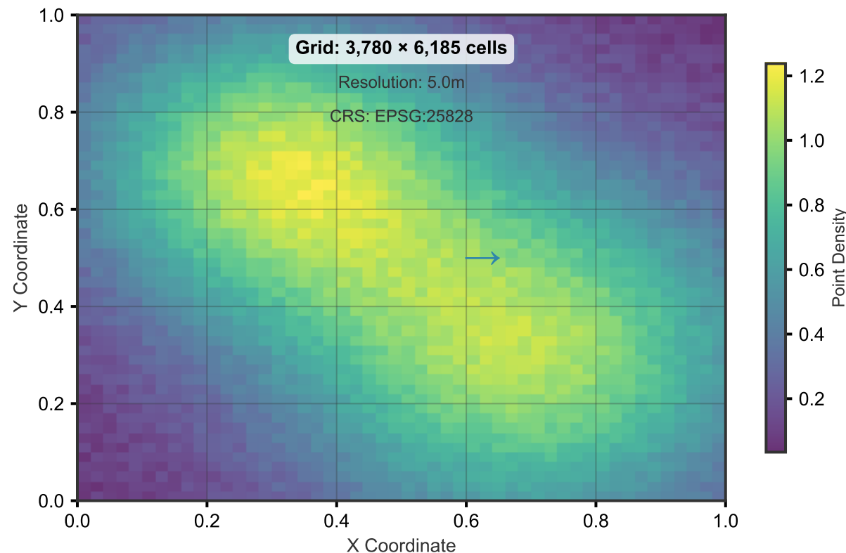
A) Raw LiDAR Point Cloud Density
