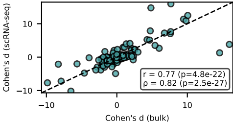
Bulk vs scRNA-seq Cohen's d
