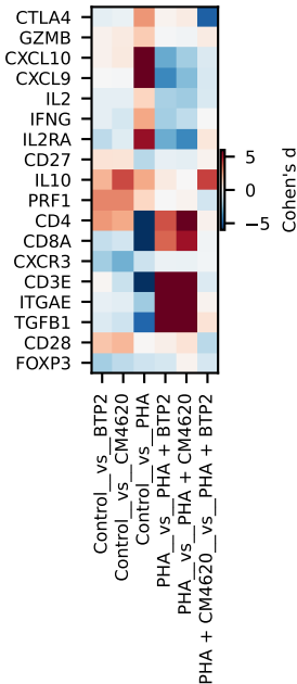
Cohen's d: scRNAseq
