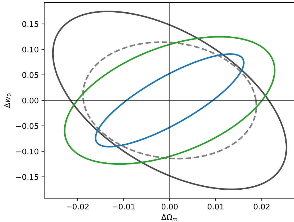
Fisher 68% contours — BARYON-SAFE regime (PS \ell_{max} = 400 ; HOS scales234, smallest scale dropped; full-sky, noisy)
