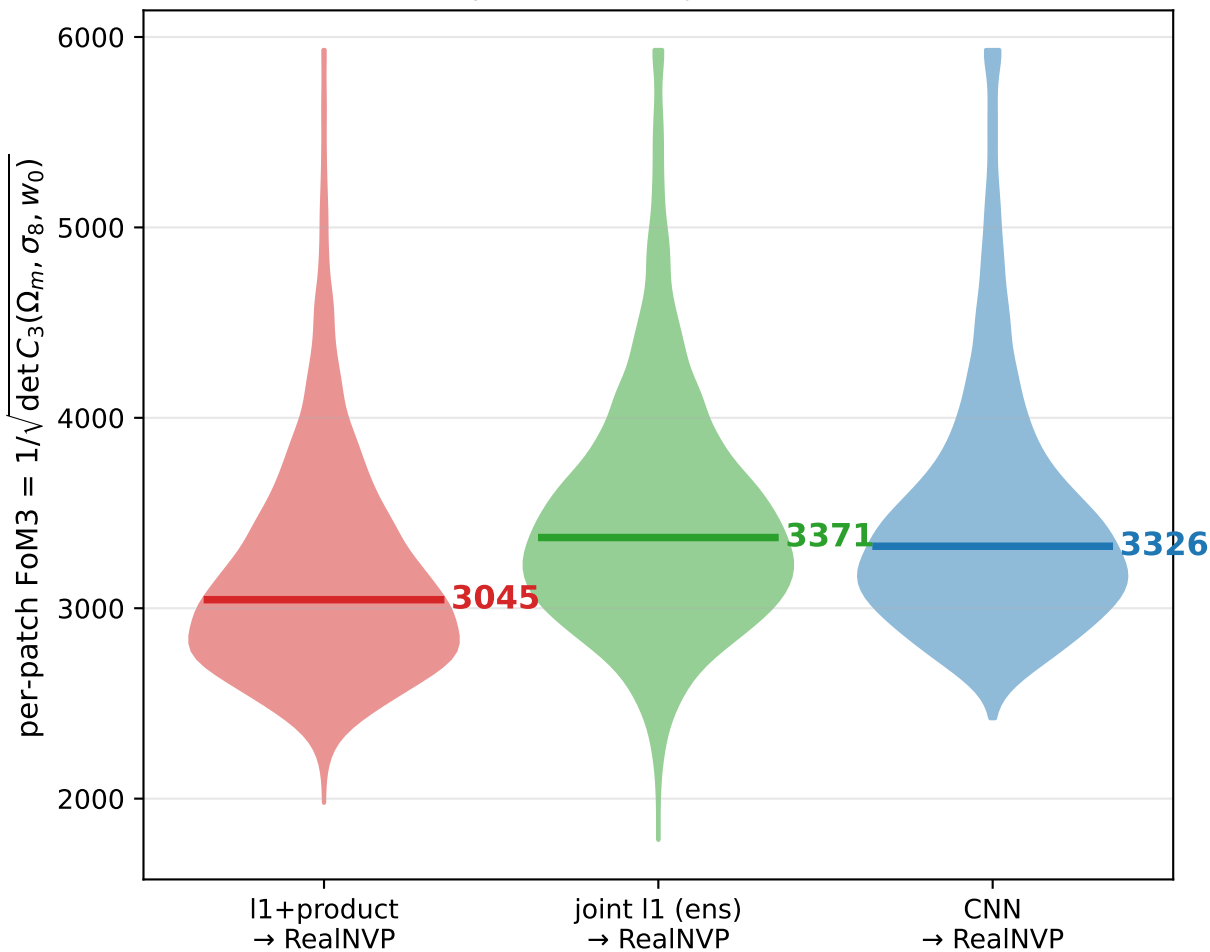
Per-patch FoM3 over the fiducial population (N=9000) medians: l1+product 3045 · joint l1 3371 · CNN 3326
