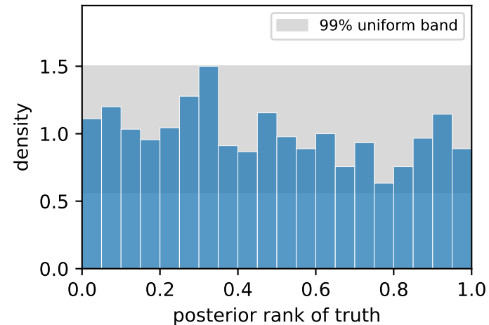
SBC — \Omega_m (1/20 out)
