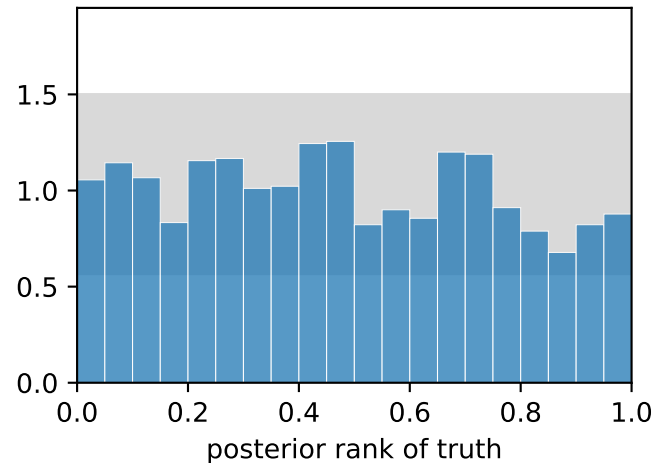
SBC — w_0 (0/20 out)
