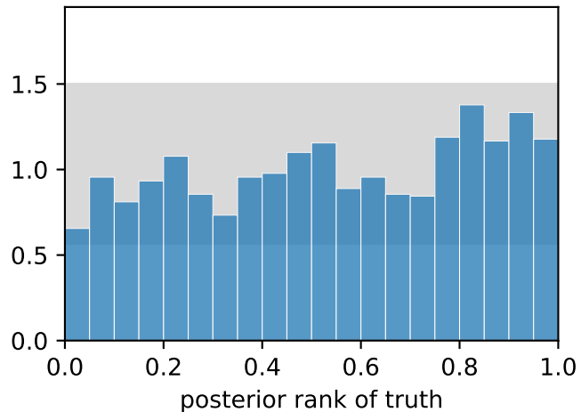
SBC — \sigma_8 (0/20 out)
