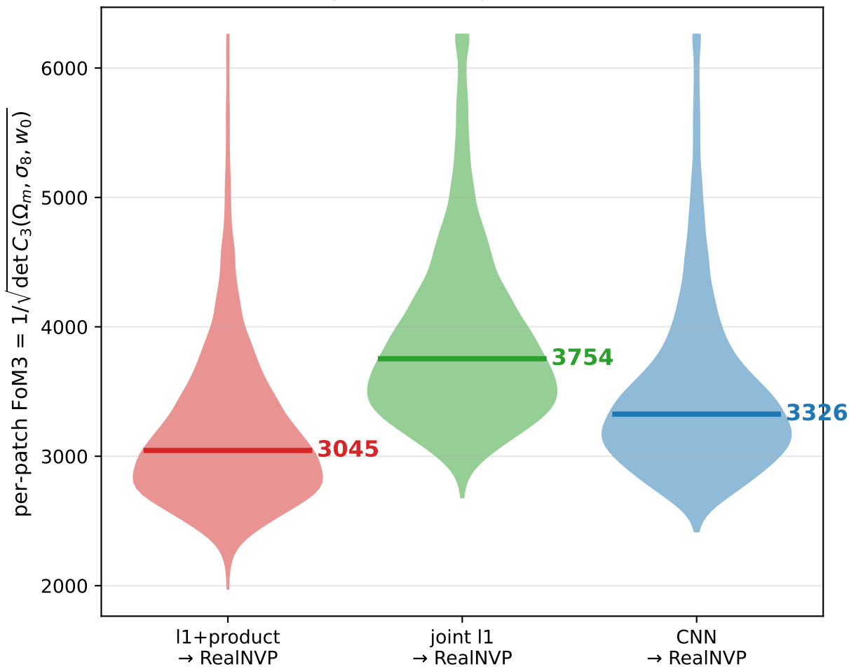
Per-patch FoM3 over the fiducial population (N=9000) medians: l1+product 3045 · joint l1 3754 · CNN 3326
