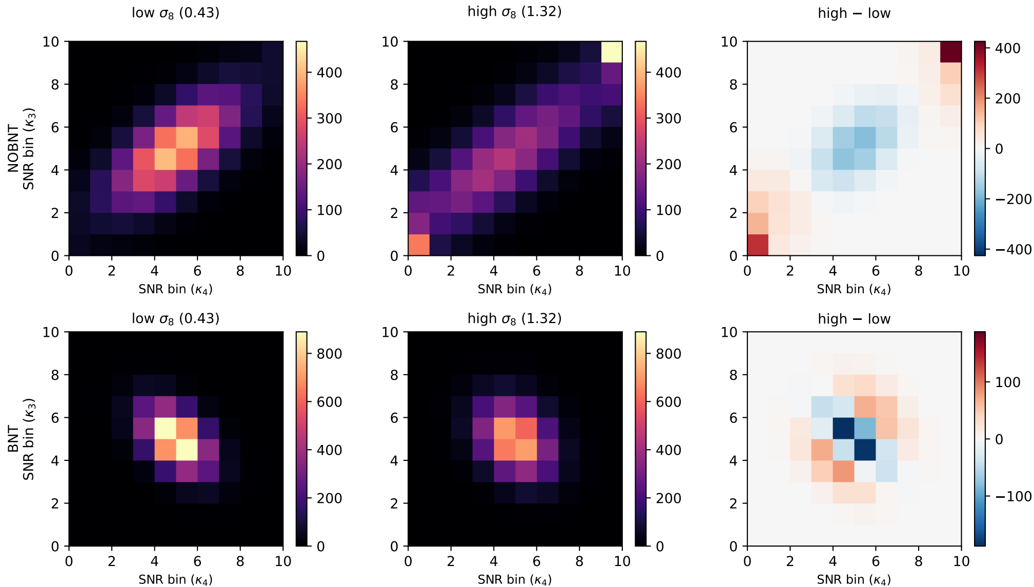
pair2dq: mean joint histogram, pair \kappa_3 \times \kappa_4 , scale 3 — low vs high \sigma_8
