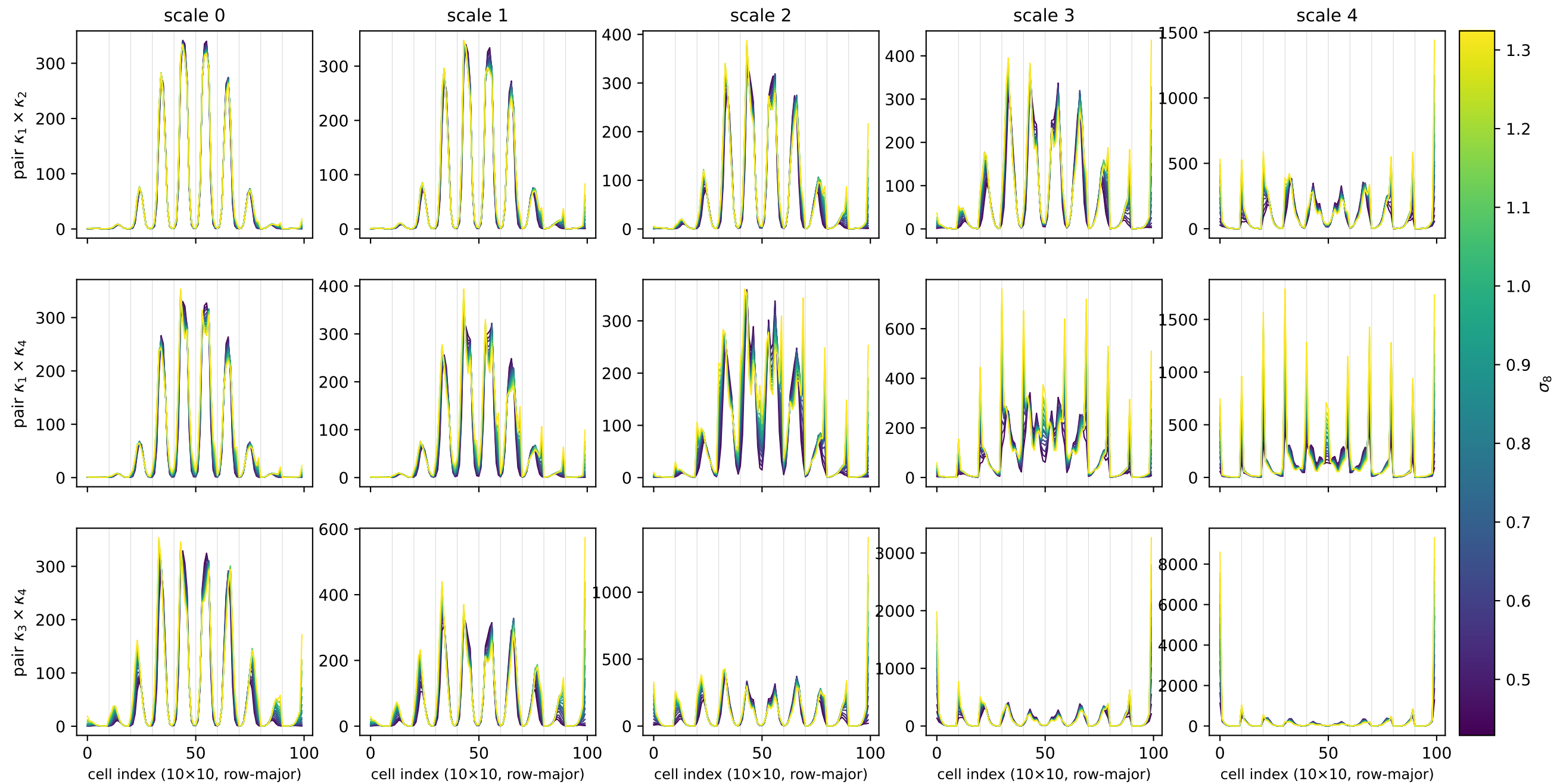
joint wavelet \ell_1 vs \sigma_8 — 16 levels, NOBNT basis (dequantized training cache)
