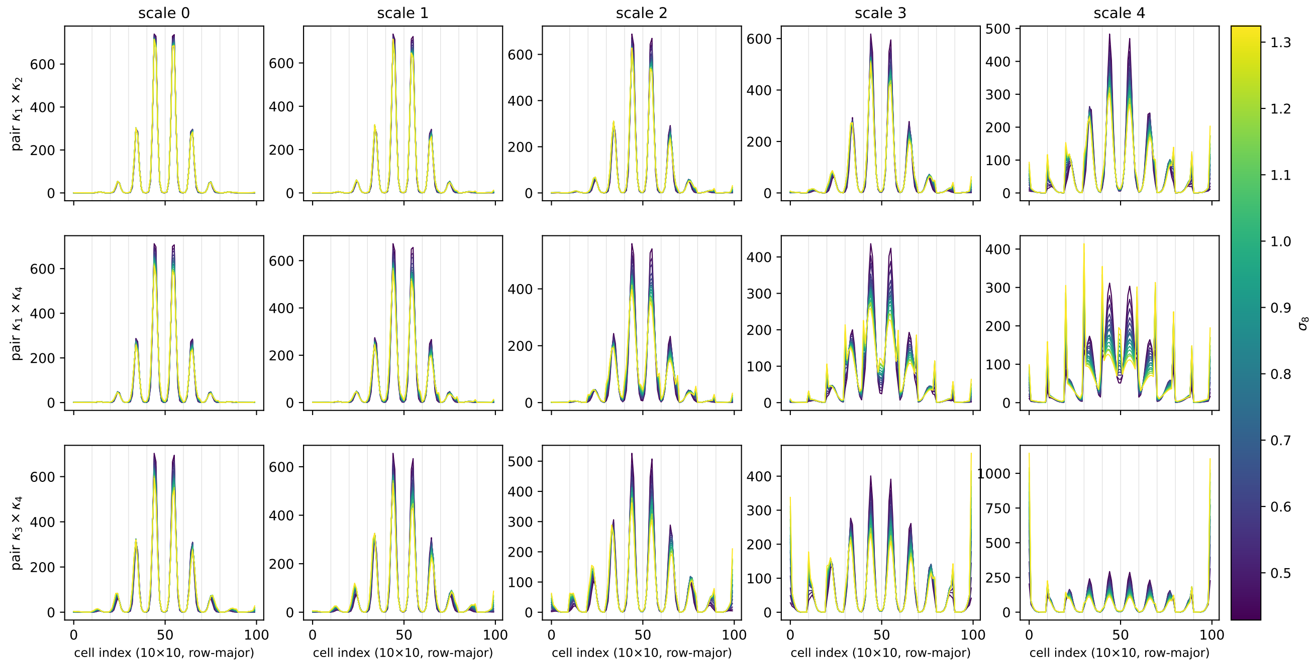
joint PDF (counts) vs \sigma_8 — 16 levels, NOBNT basis (dequantized training cache)
