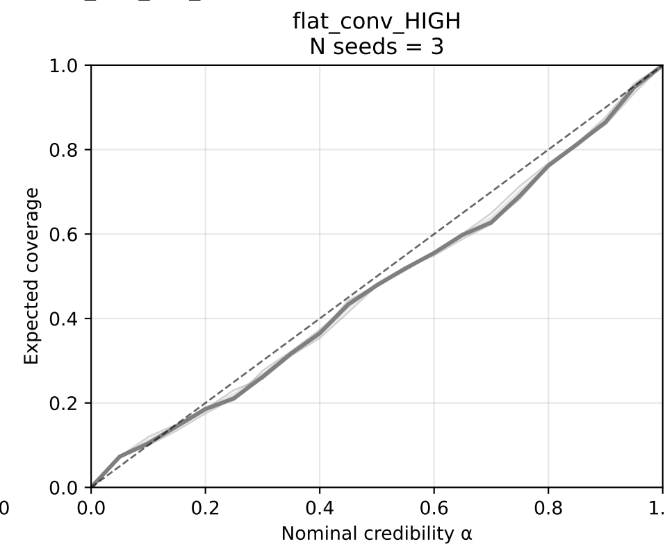
TARP coverage — 3-D ( \Omega_m, \sigma_8, w_0 )
