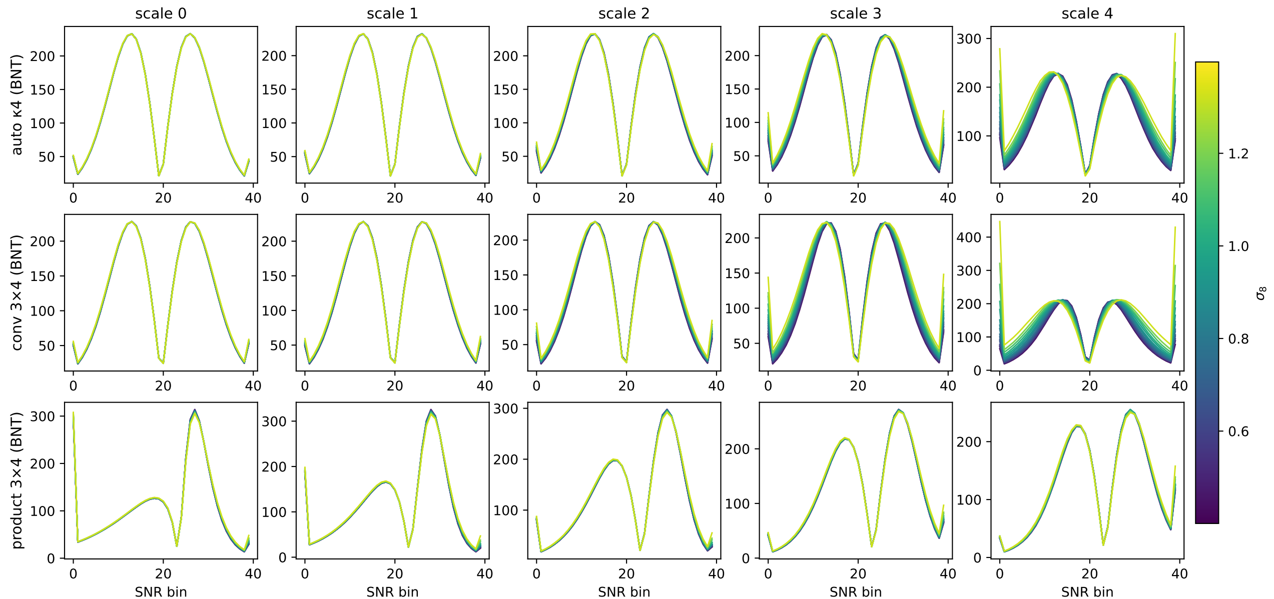
L1 histograms vs \sigma_8 — 16 cosmology levels (op=both, exact datavector, BNT basis)
