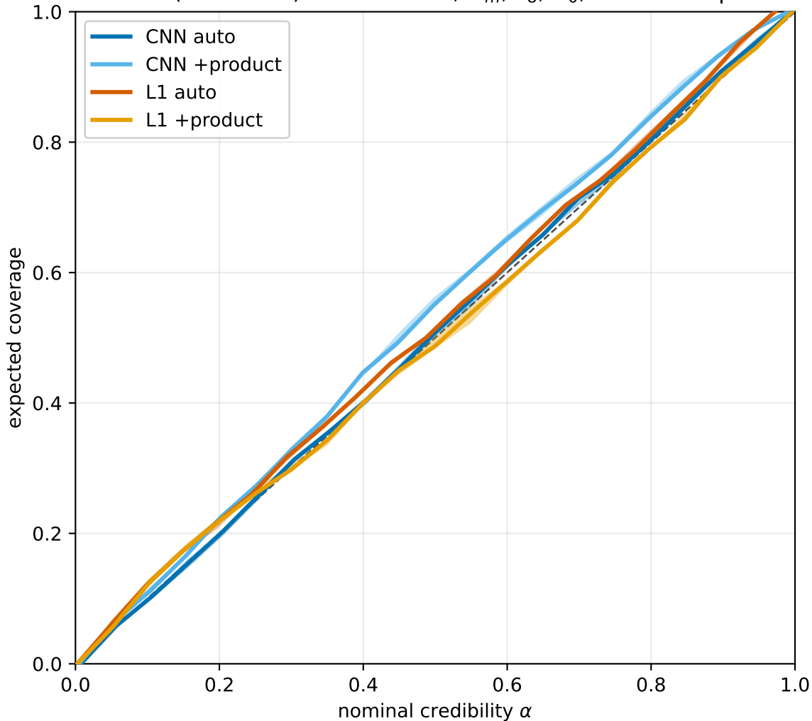
GATE C (BNT arms) — TARP-DRP, \Omega_m , \sigma_8 , w_0 , all 600 val points
