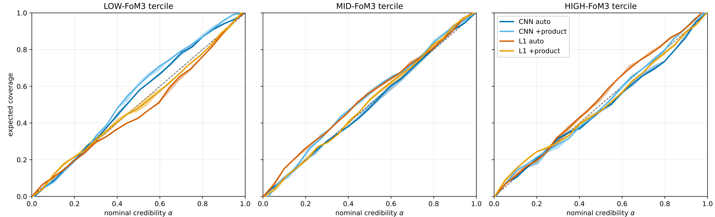
GATE C (BNT arms) — TARP-DRP, \Omega_m , \sigma_8 , w_0 (band = 16-84% over 3 seeds \times 200 bootstraps)
