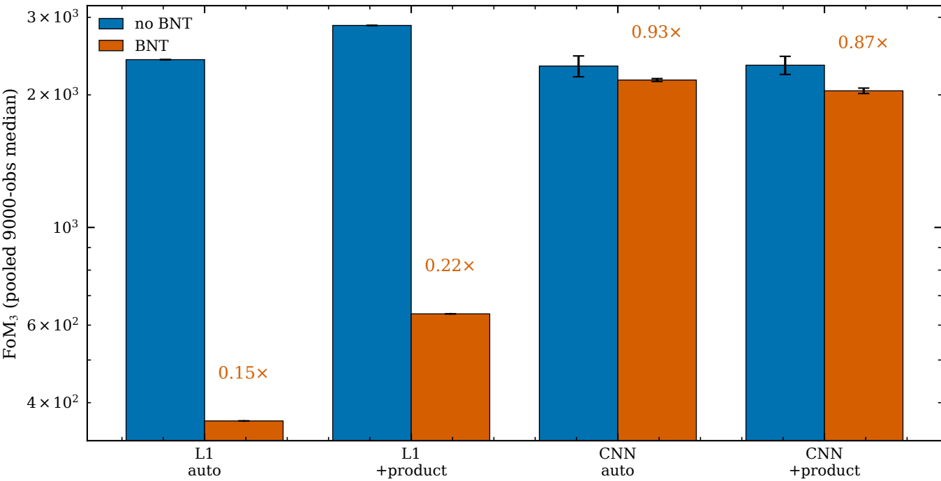
BNT inflation: per-channel L1 collapses, the CNN is (near-)lossless
