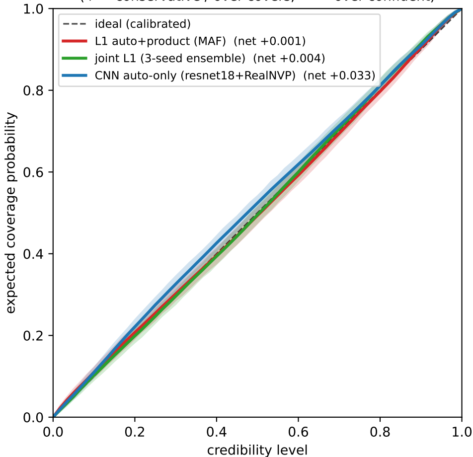
TARP-DRP, un-stratified, 1\sigma bands (+ = conservative / over-covers; - = over-confident)
