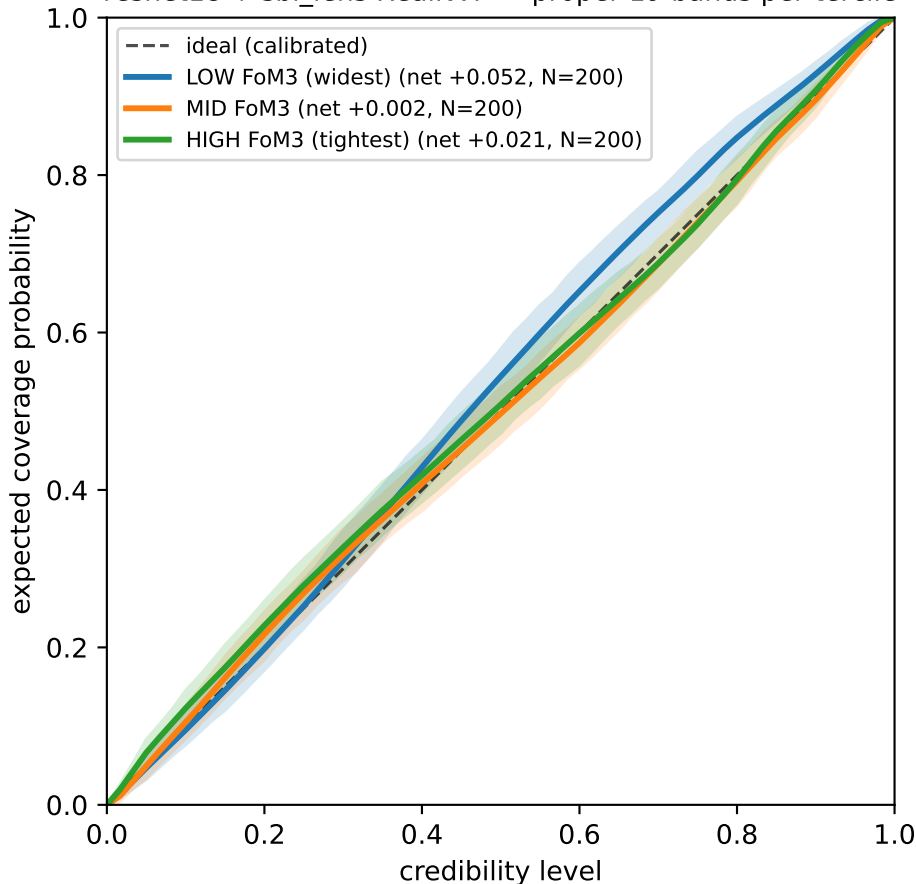
CNN TARP-DRP, FoM3-stratified (like-with-like) resnet18 + sbi_lens RealNVP · proper 1\sigma bands per tercile
