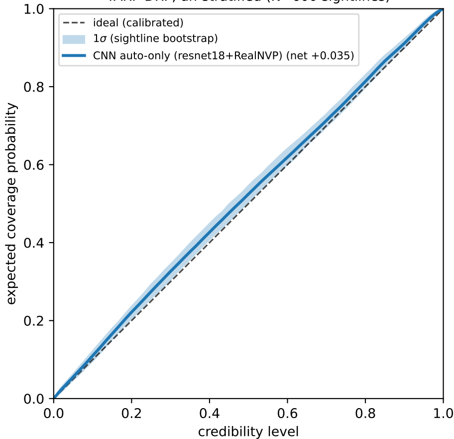
TARP-DRP, un-stratified (N=600 sightlines)
