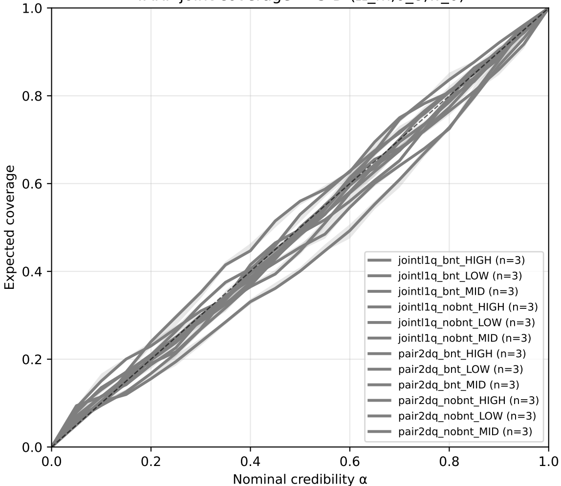
TARP joint coverage — 3-D ( \Omega_m, \sigma_8, w_0 )
