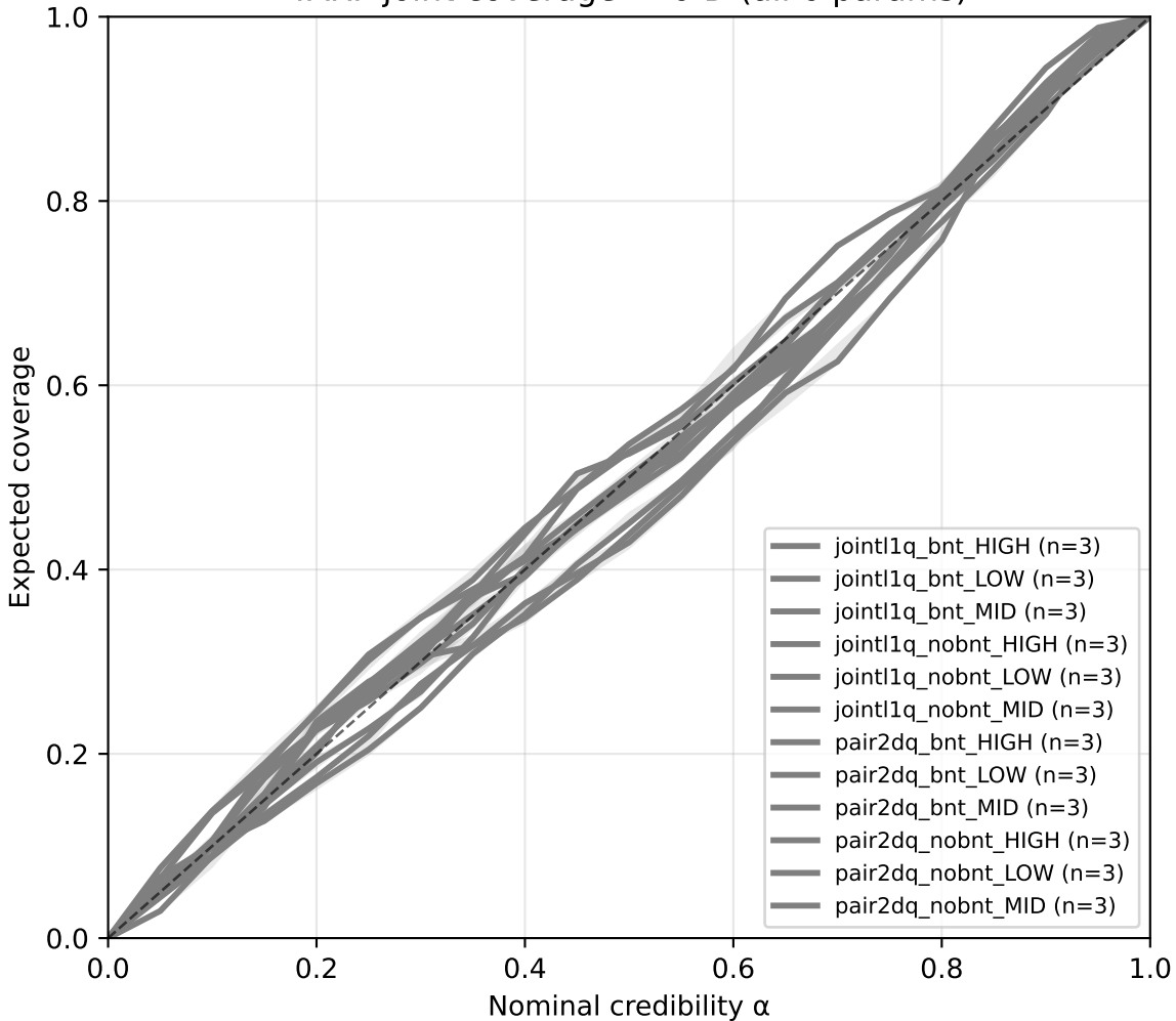
TARP joint coverage — 6-D (all 6 params)
