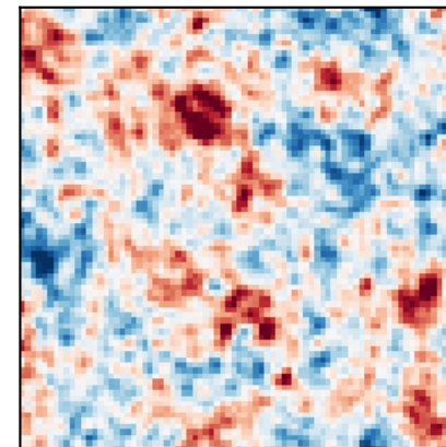
product 3×4
