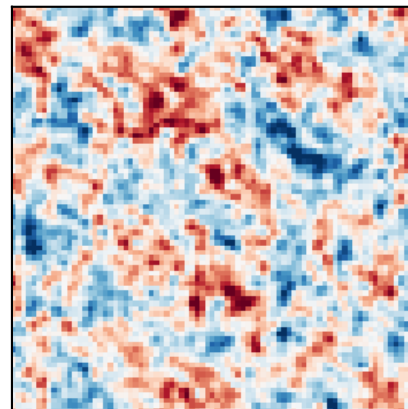
product 2×3
