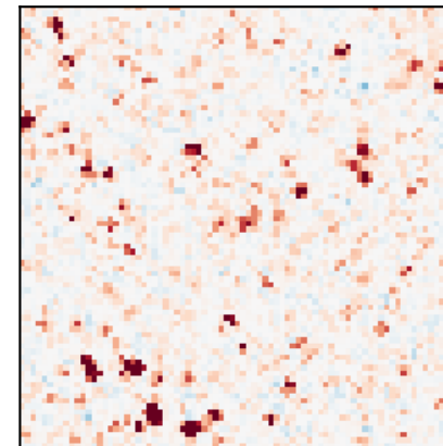
product 3×4
