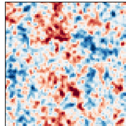
product 2×4
