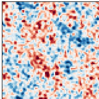
product 1×4
