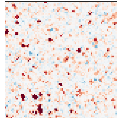
product 2×4
