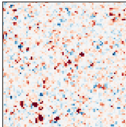
product 1×4
