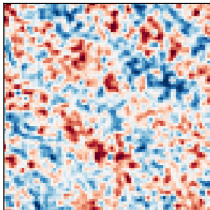
product 1×3
