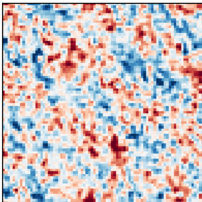
product 1×2
