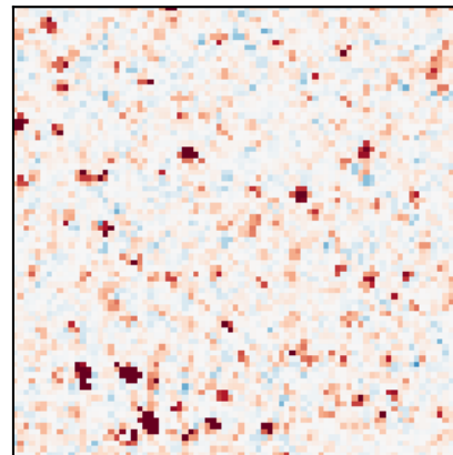
product 2×3
