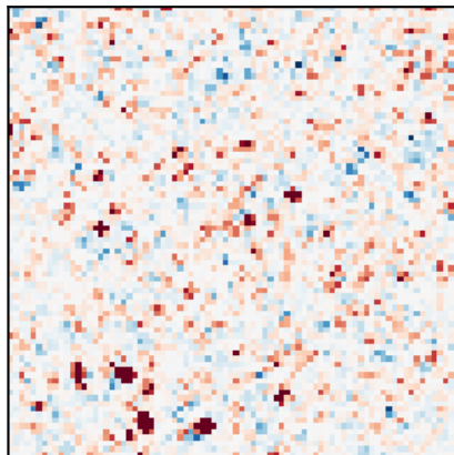
product 1×3
