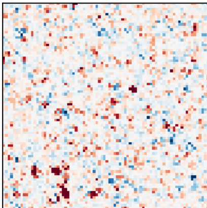
product 1×2
