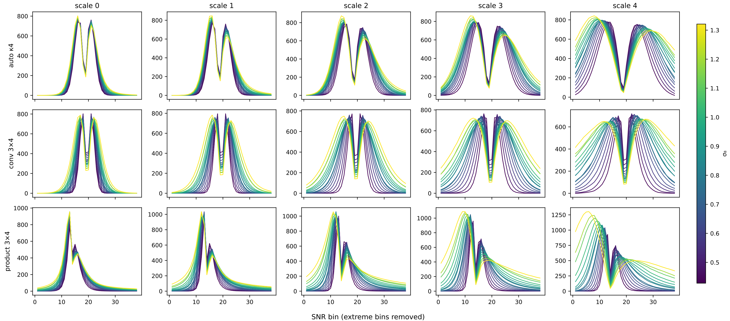
L1 histograms vs \sigma_8 — 16 cosmology levels (op=both, exact datavector)
