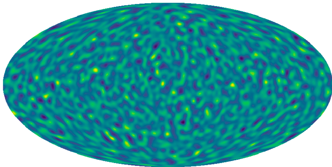
Wavelet 4
