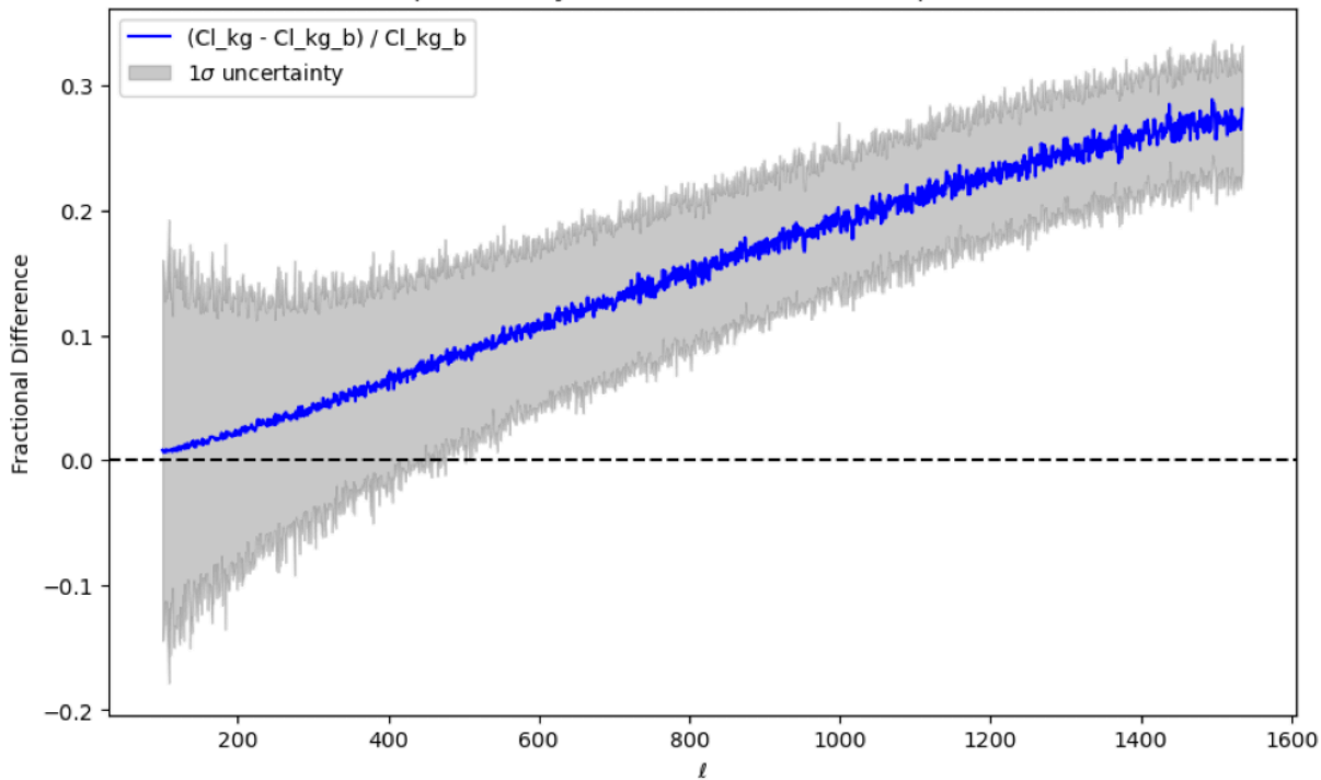
Impact of Baryonic Effects on the Power Spectrum
