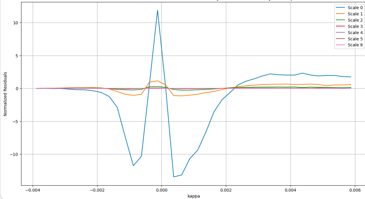
Normalized Residuals of the l1-norms between Baryonified and Non-baryonic Maps
