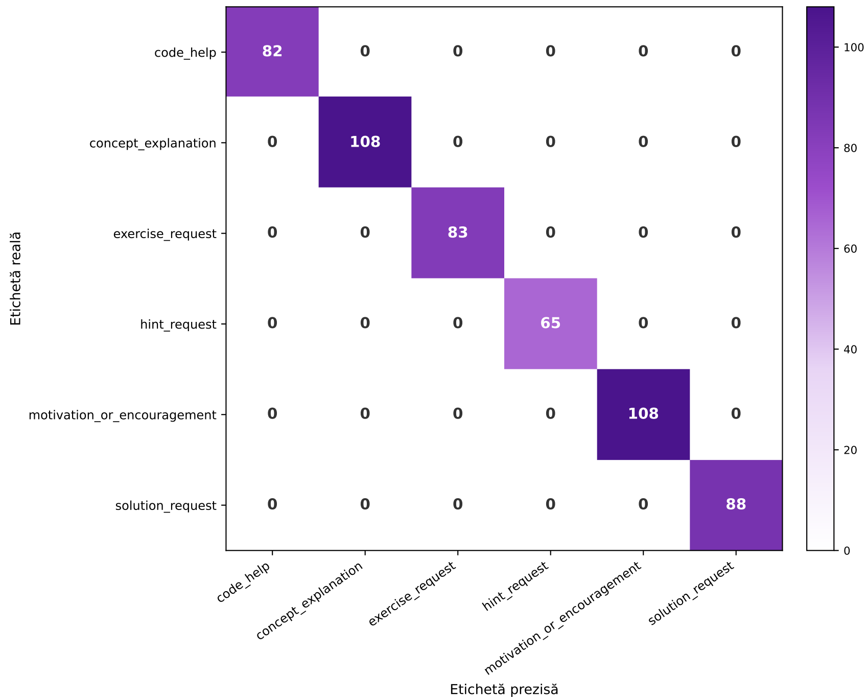
BERT Românesc varianta 2 — Label Acc=100.00% F1=100.00%
