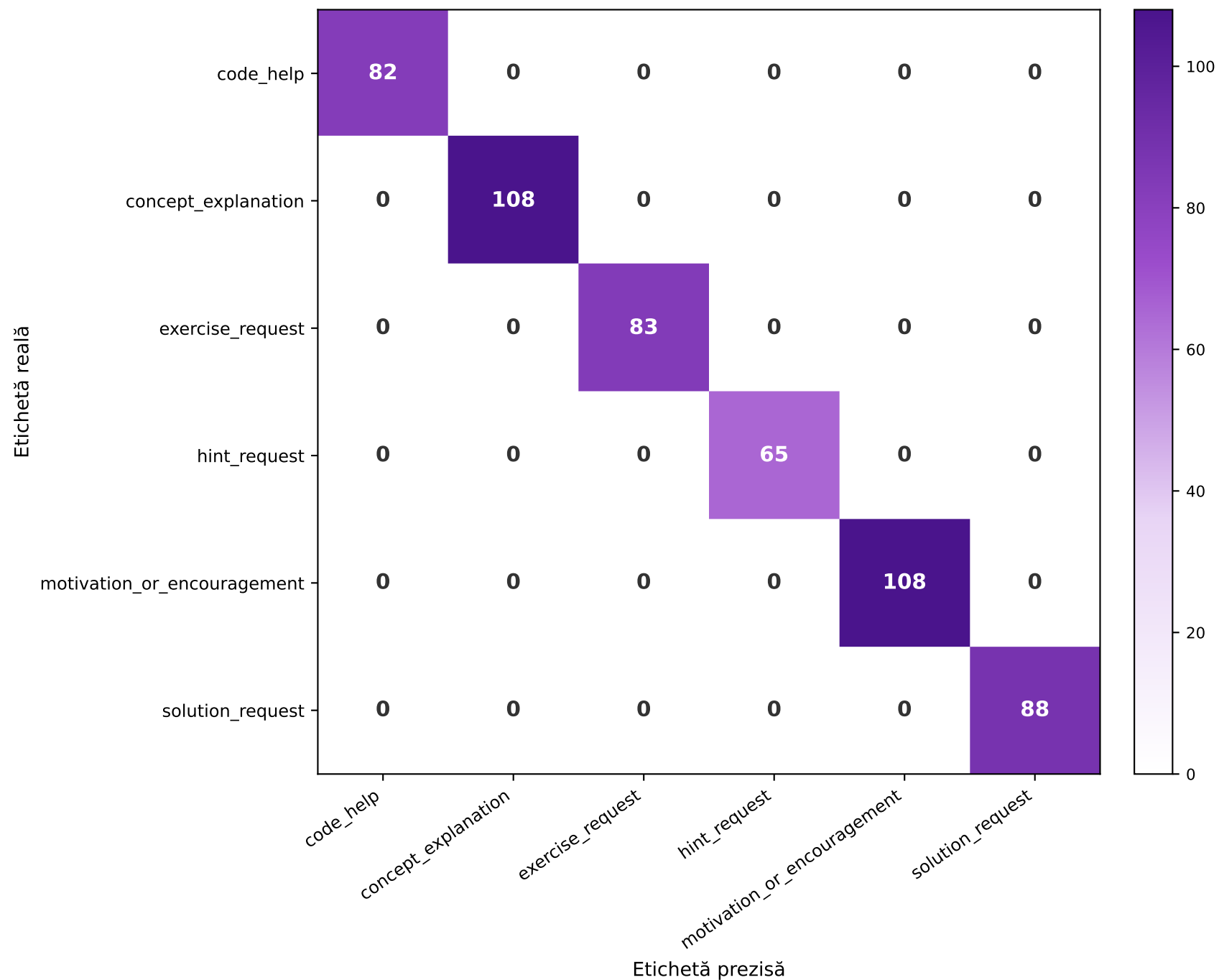
Ensemble (RoBERT + BERT v2) — Label Majority Voting | Acc=100.00% F1=100.00%
