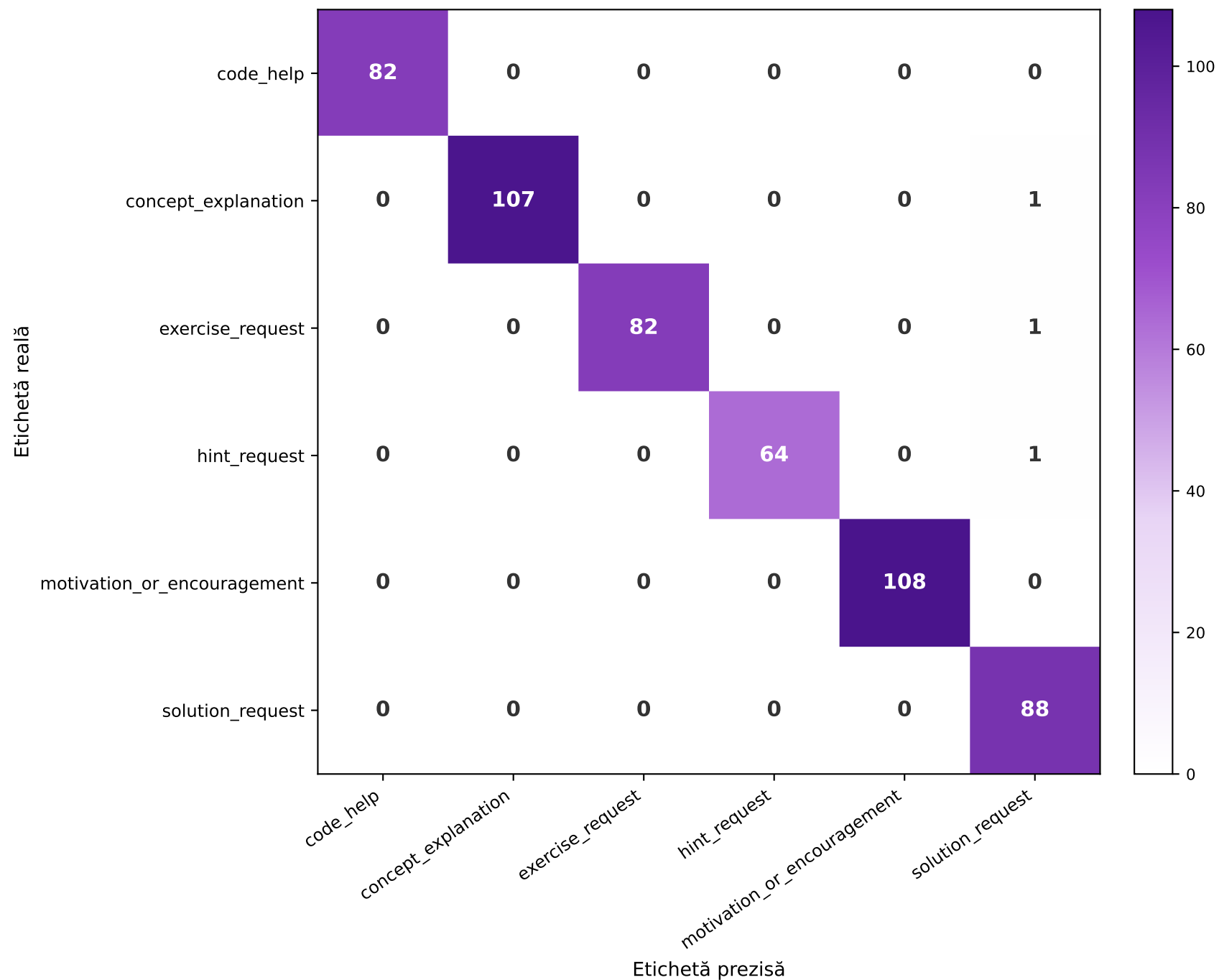
XLM-RoBERTa varianta 1 — Label Acc=99.44% F1=99.41%
