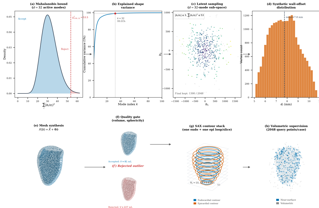
Figure 3.3. Synthetic ED dataset generation, from SSM sampling to geometric supervision. Top row, statistical constraints: (a) distribution of the overall-deviation (Mahalanobis) statistic of Equation (3.2) with the \chi^2_{0.99,32} acceptance threshold; (b) cumulative shape variance, with 32 active modes reaching 99%; (c) accepted coefficient samples in the first two modes; (d) distribution of the synthetic epicardial offset of Equation (3.3). Bottom row, geometric construction: (e) mesh synthesis via Equation (3.1); (f) an accepted shape next to a rejected outlier; (g) the 10 SAX contour levels; (h) the 2048 near-surface and volumetric query points used for decoder supervision.
