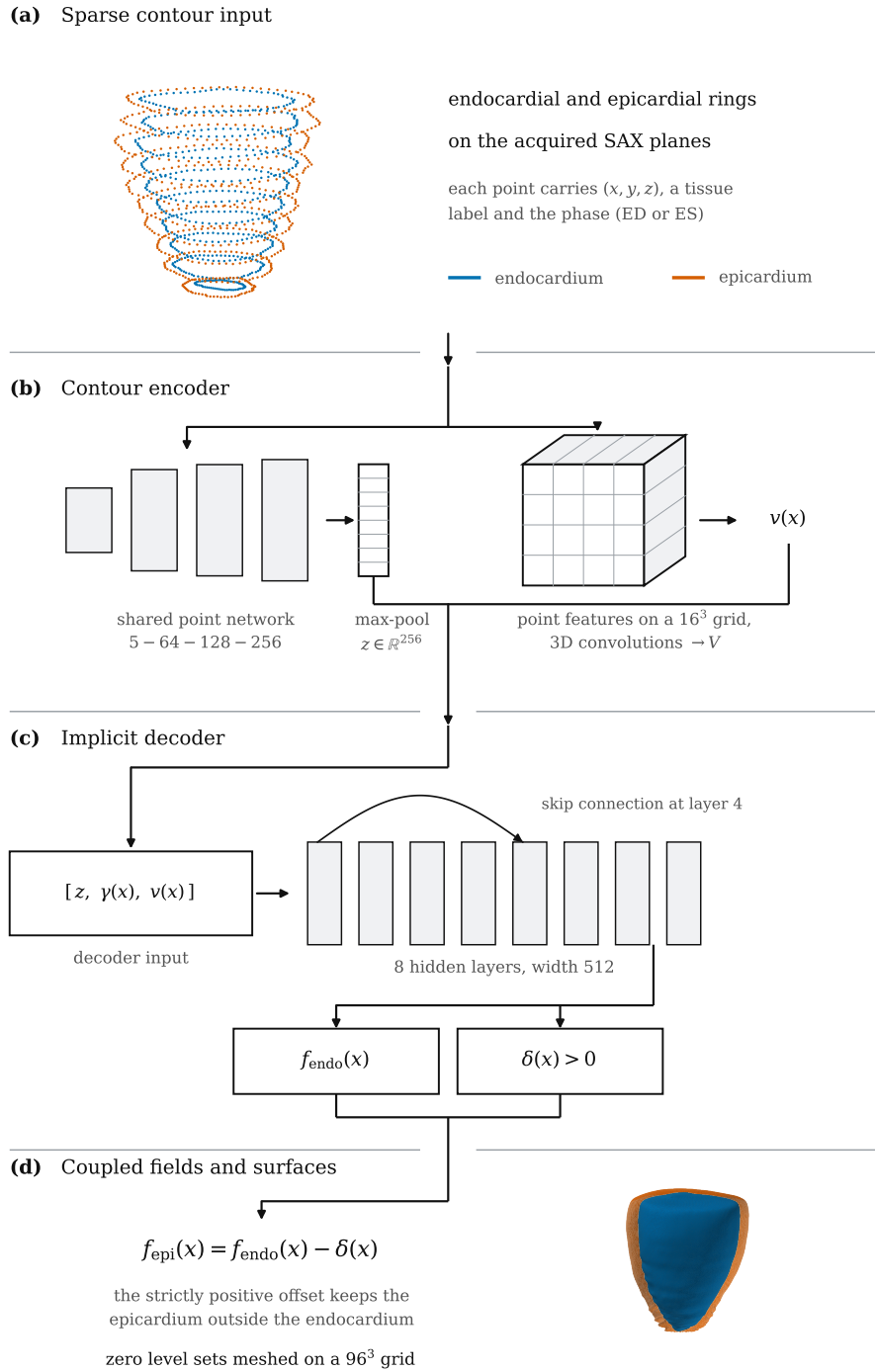
Figure 3.7. Phase-conditioned model architecture, from the sparse contour observation (a) through the global and local encoder paths (b) and the implicit decoder (c) to the coupled fields and extracted surfaces (d). The point cloud in (a) and the cut surfaces in (d) are the observed contours and the corresponding reconstruction of one ACDC case, with the epicardium opened to expose the endocardial cavity.
