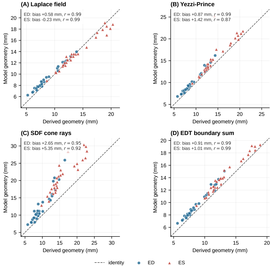
Figure 4.4. Patient-level mean wall thickness on model and segmentation-derived geometry at ED and ES. The dashed identity line denotes equal values; annotations report model-minus-comparator bias and Pearson correlation.
