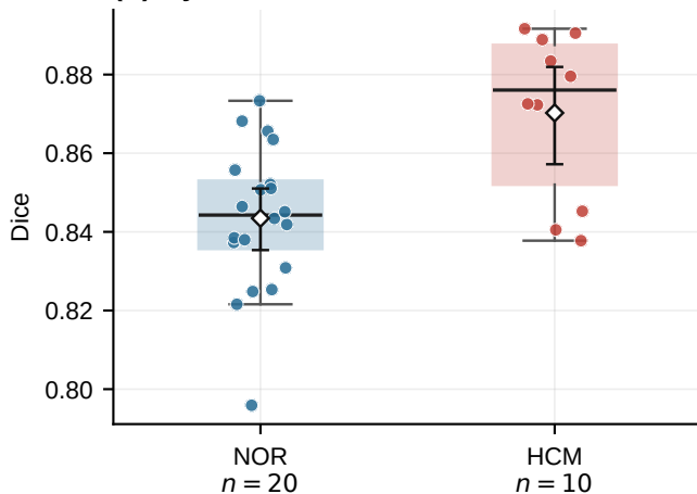
(C) Myocardial Dice
