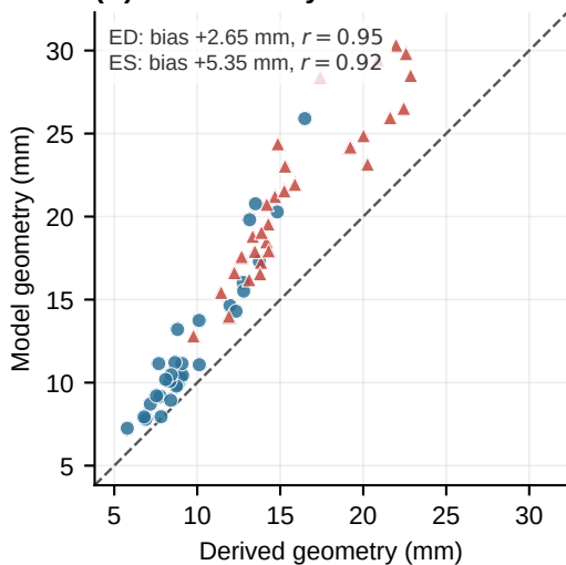
(C) SDF cone rays
