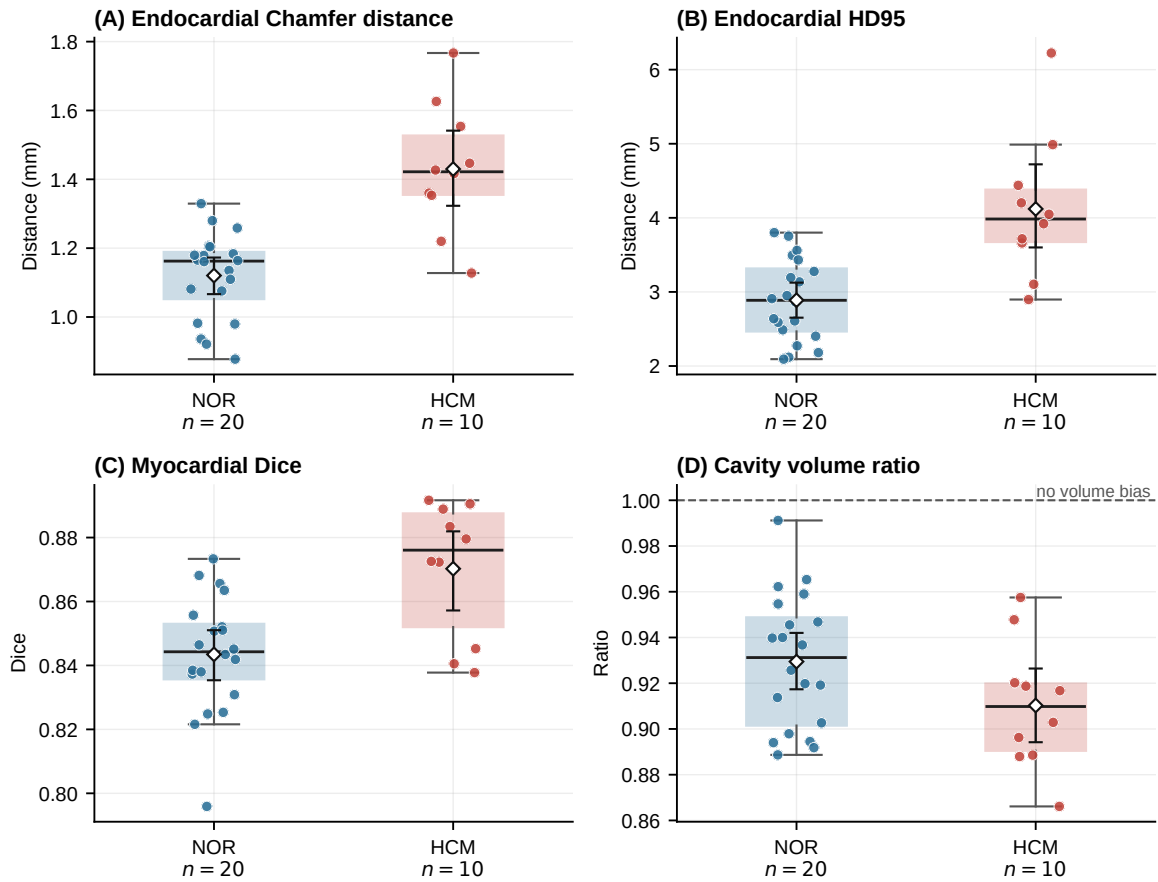
Figure 4.4. Patient-level end-diastolic reconstruction metrics for the normal and HCM groups. Points represent patients; diamonds and bars show group means with 95% bootstrap confidence intervals.
