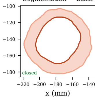
Segmentation — basal
