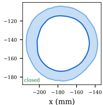
CardioSDF — mid
