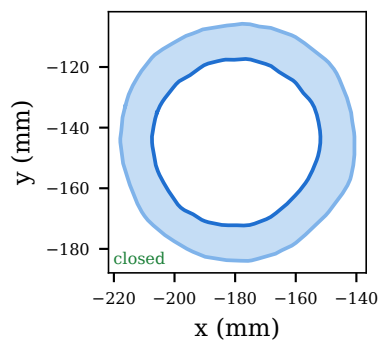
CardioSDF — basal
