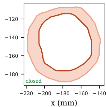
Segmentation — mid
