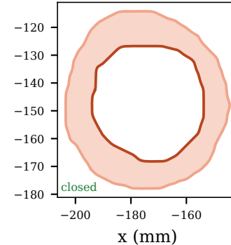
Segmentation — apical
