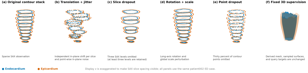
FIGURE 3.7. Contour-input augmentation applied to every training data stream. Each panel starts from the same ACDC patient002 ED contour stack; colours identify endocardial (blue) and epicardial (orange) points. The operations show representative draws of per-slice translation with point jitter, slice dropout, long-axis rotation with global scale jitter, and contour-point dropout. Only the encoder observation changes. The derived endocardial and epicardial meshes, supervision samples, query points, tissue labels, and phase label remain attached to the original case.
