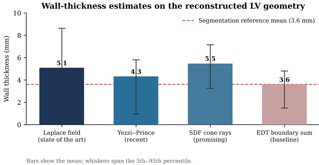
FIGURE 4.1. Mean wall thickness of the four selected methods on the reconstructed LV geometry, with whiskers spanning the 5th to 95th percentile. The dashed line marks the mean wall thickness measured directly from the input segmentation.
