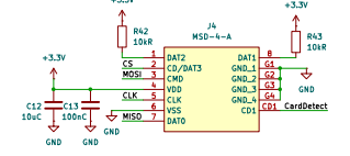
microSD card
