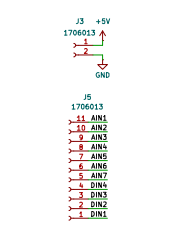
Sense and Power Headers
