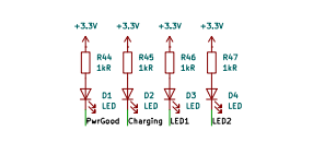
Debug & Status LEDs
