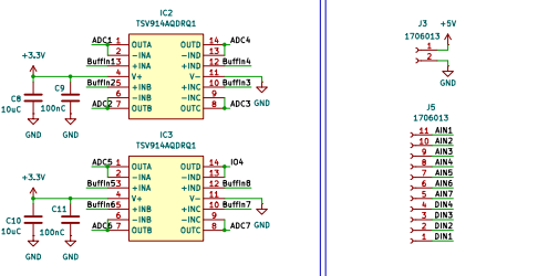
Analog Sense Attenuation
