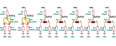
Digital Sense Attenuation
