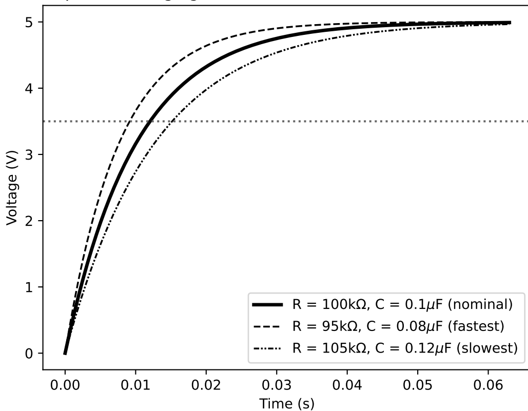
Capacitor charging under R ( \pm 5\% ) and C ( \pm 20\% ) tolerance
