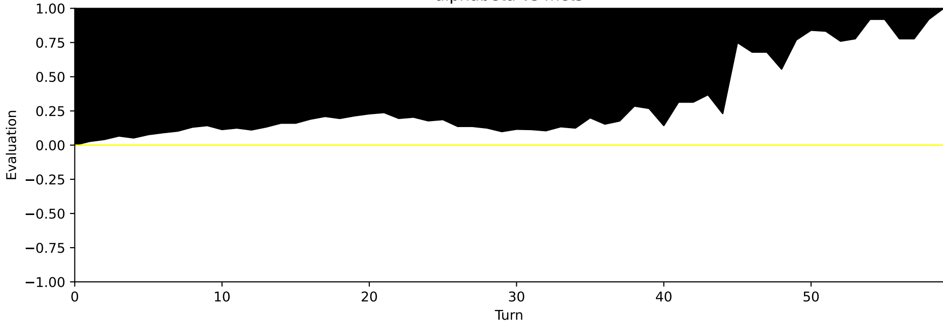
Game 1 Evaluation alphabetalpha vs mcts
