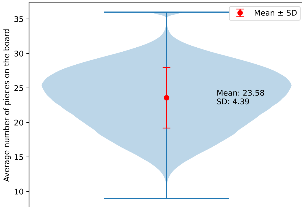
Average number of pieces on the board during a game
