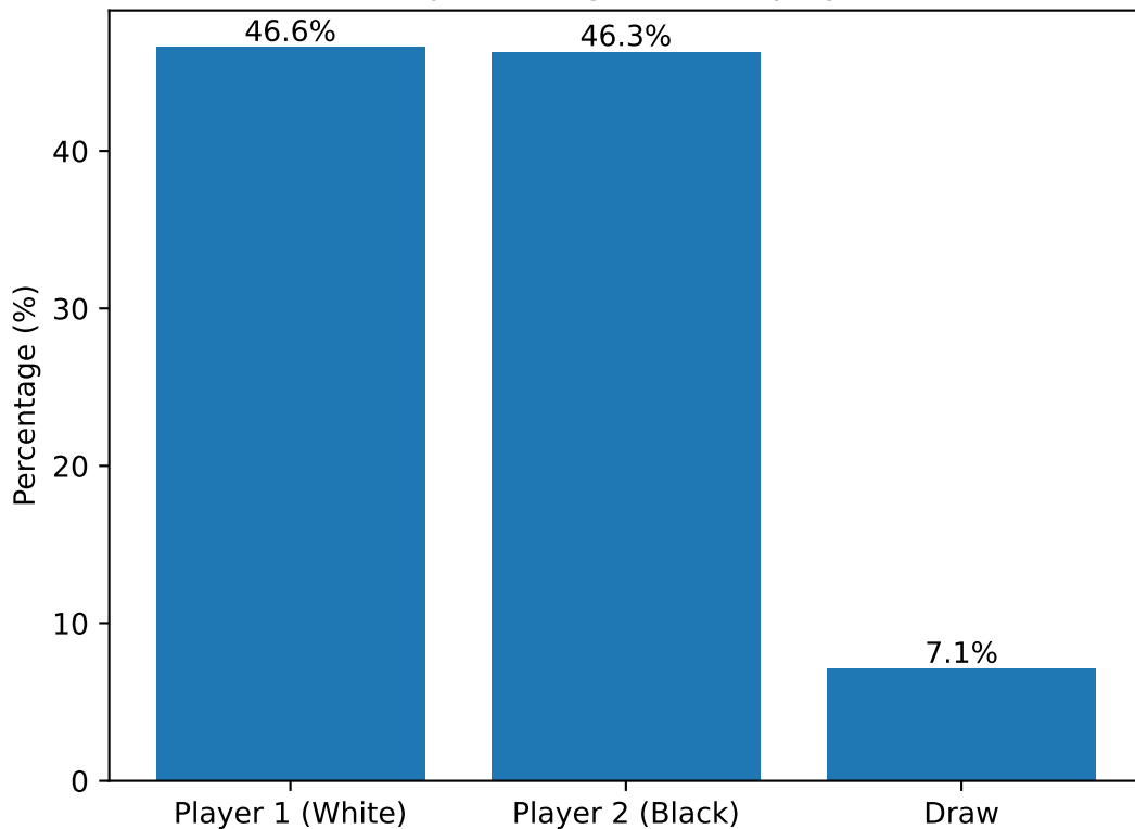
Win percentages (%) of players
