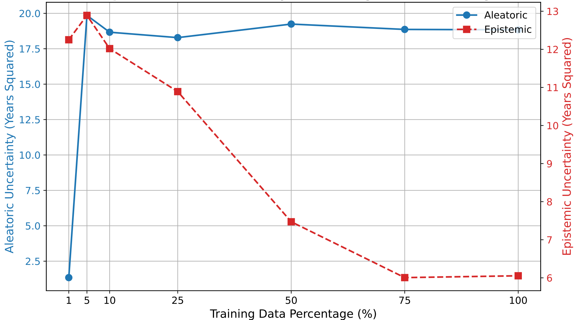
Dropconnect — Uncertainty vs Training Data Percentage
