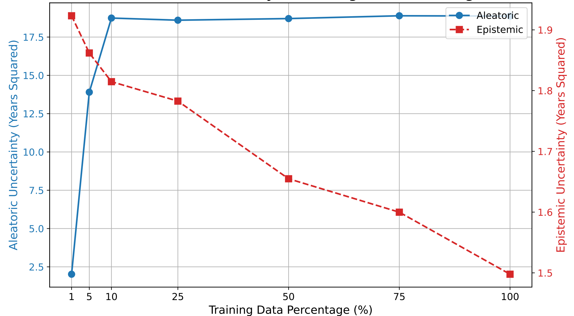
Ensemble — Uncertainty vs Training Data Percentage
