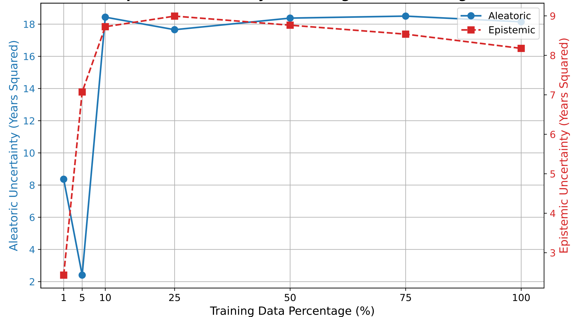
Flipout — Uncertainty vs Training Data Percentage
