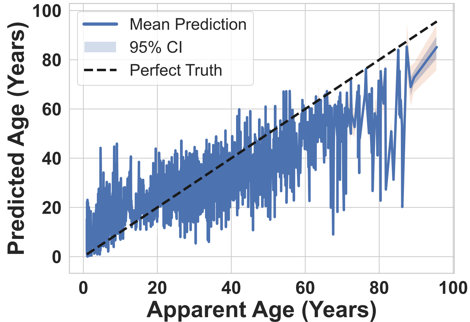
DropConnect – Epistemic Uncertainty
