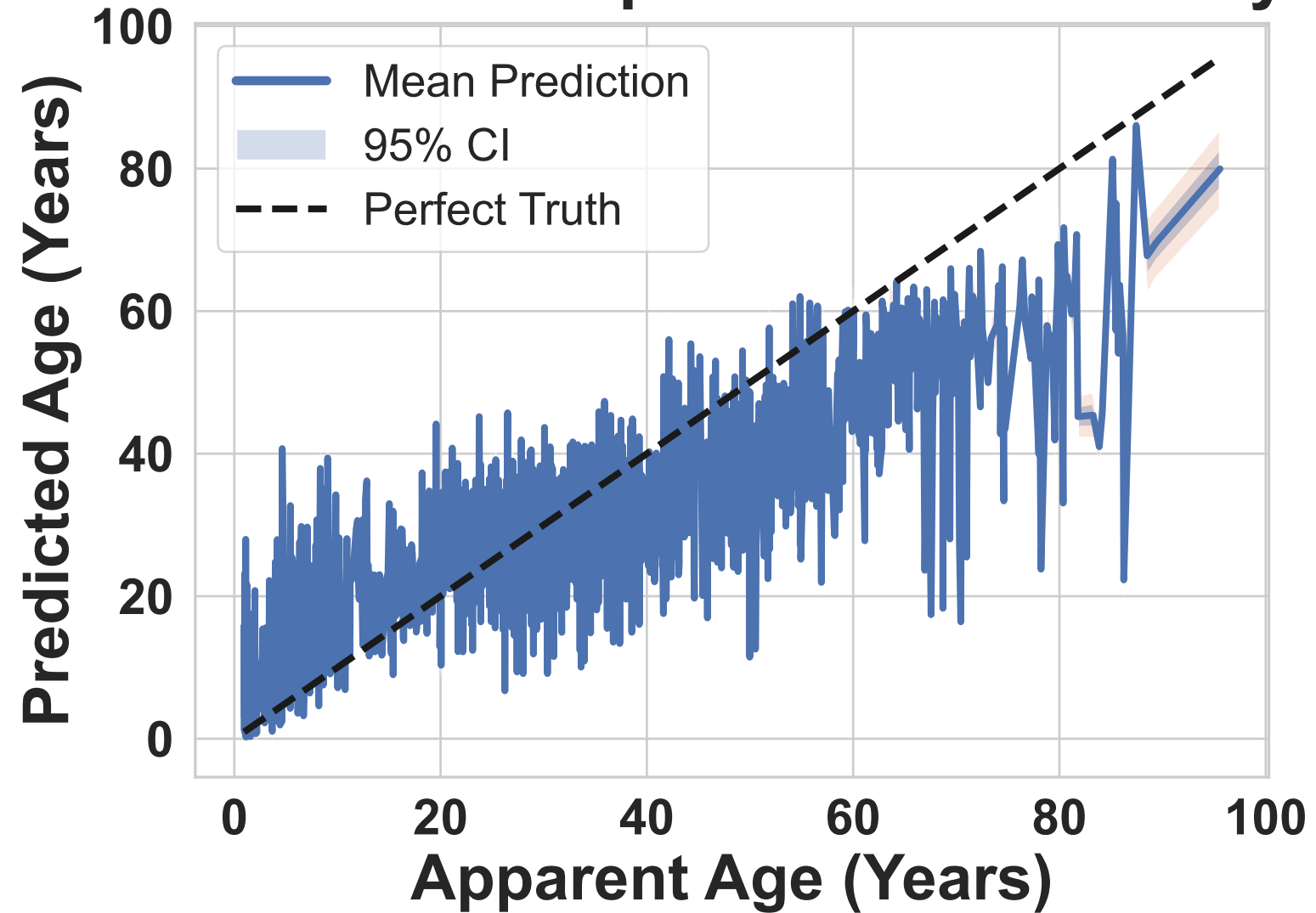
Ensemble – Epistemic Uncertainty
