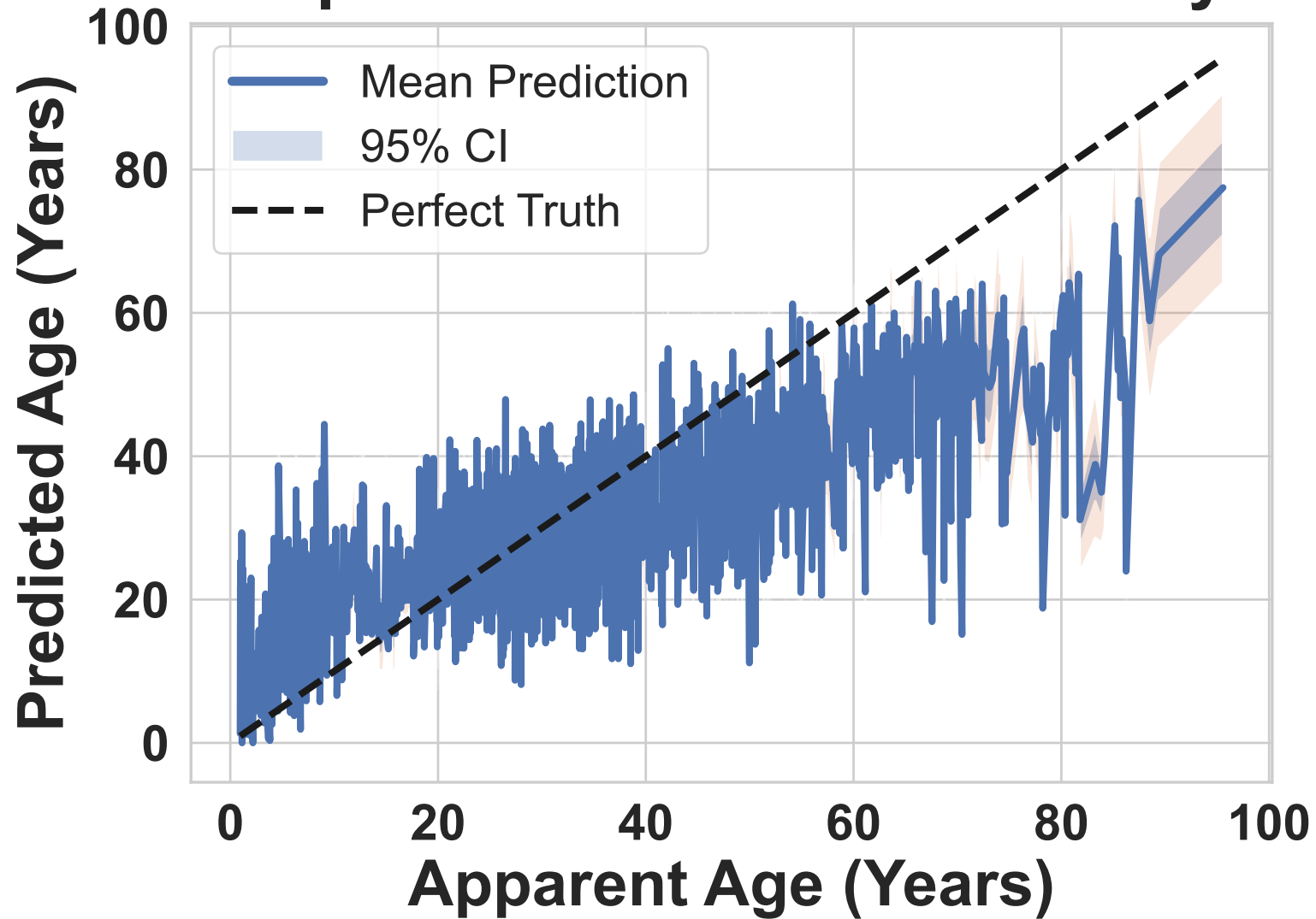
Flipout – Aleatoric Uncertainty
