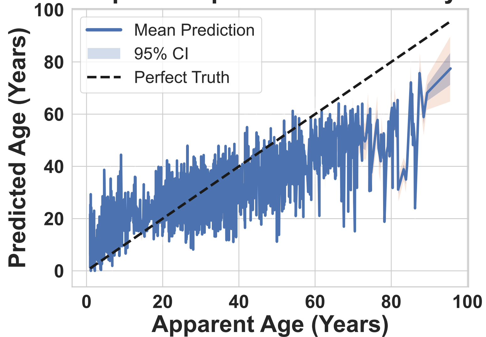
Flipout – Epistemic Uncertainty
