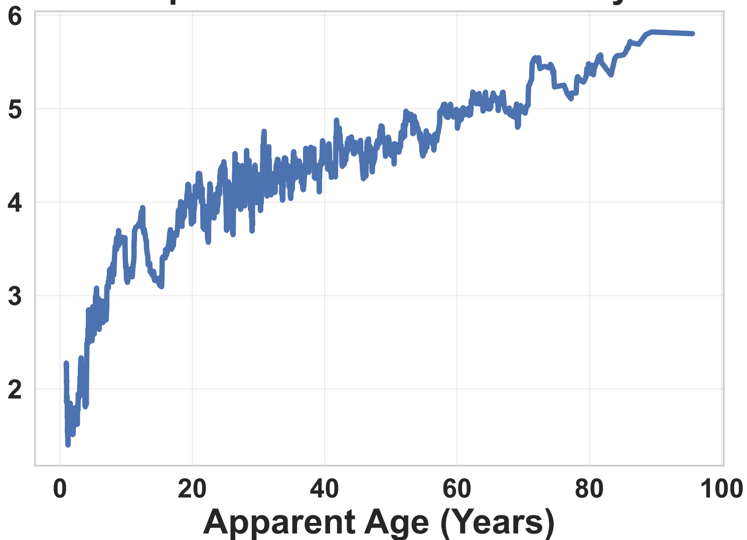
Flipout – Epistemic / Total
