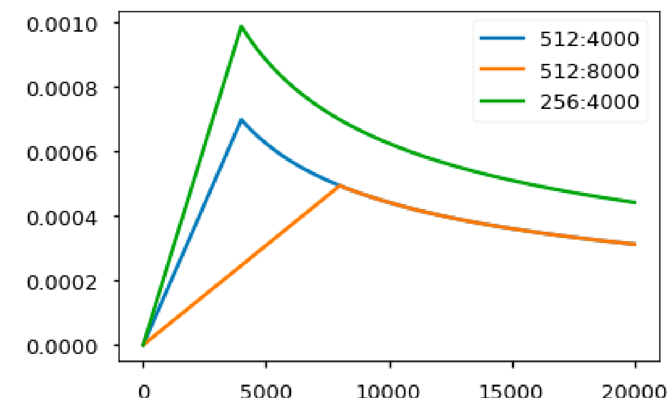
lr schedule
