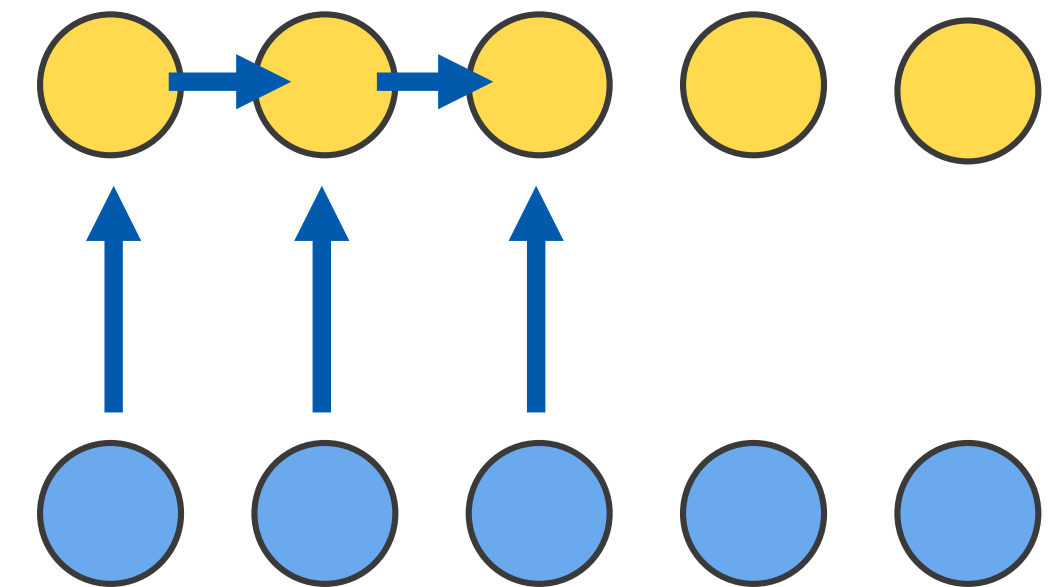
Recurrent
