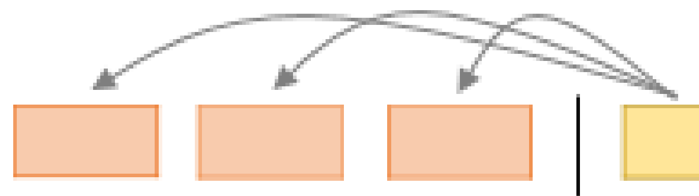
Encoder-Decoder Attention
