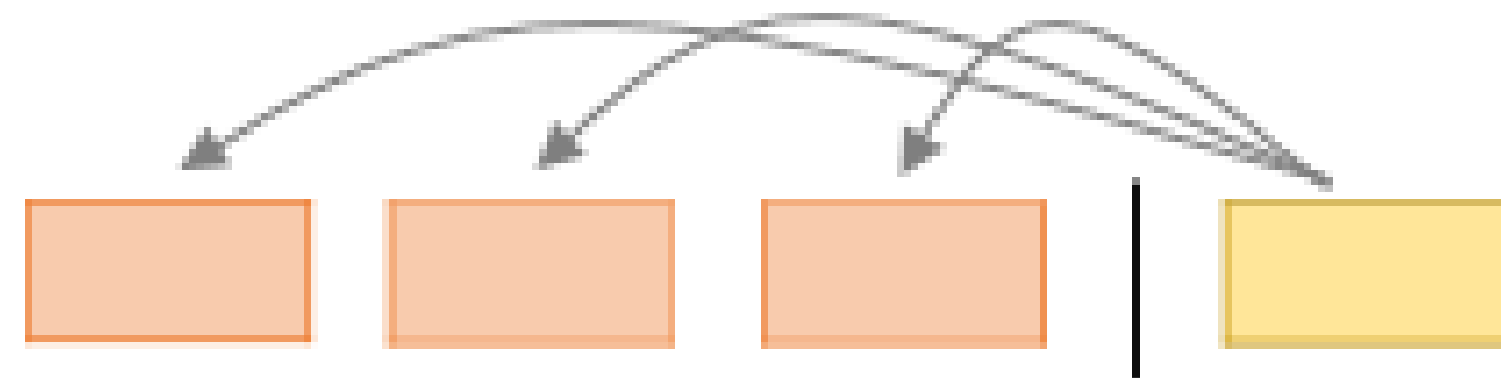
Encoder-Decoder Attention
