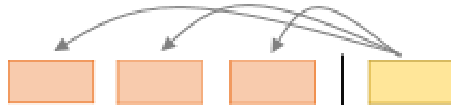
Encoder-Decoder Attention
