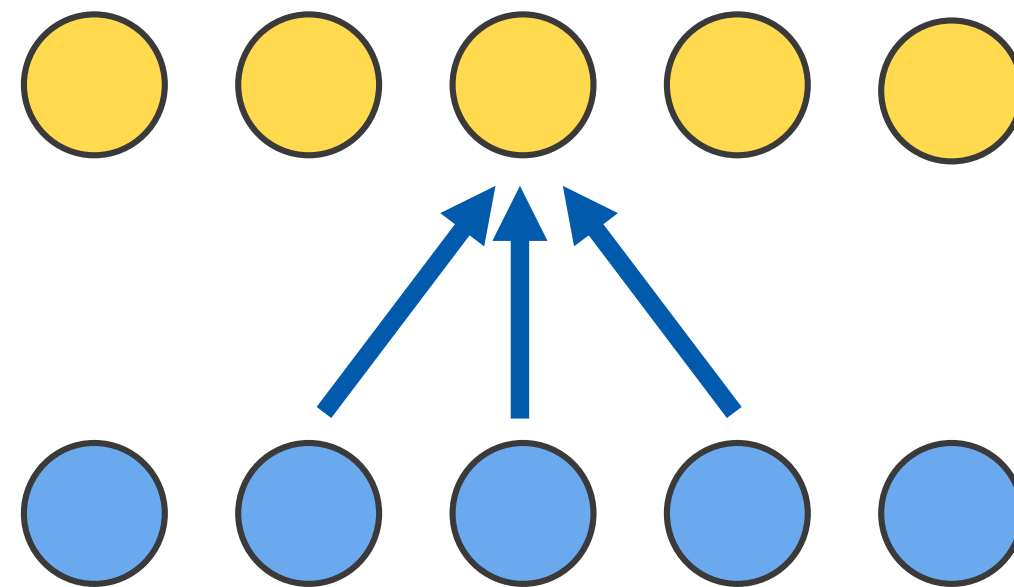
Convolutional
