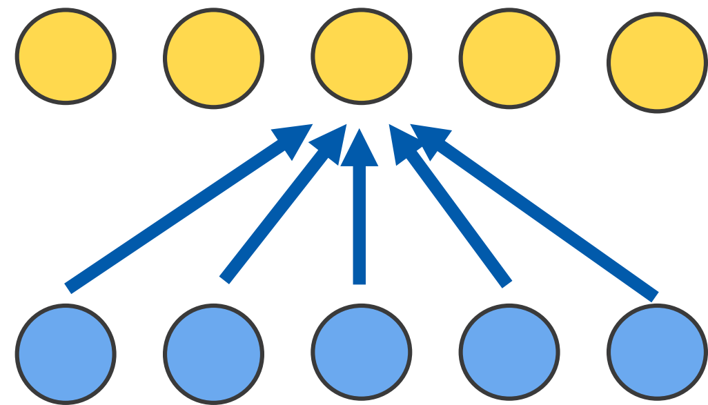
Fully-connected
