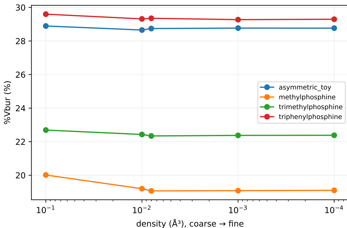
Frozen StericX convergence: odd-grid regional bias is retained
