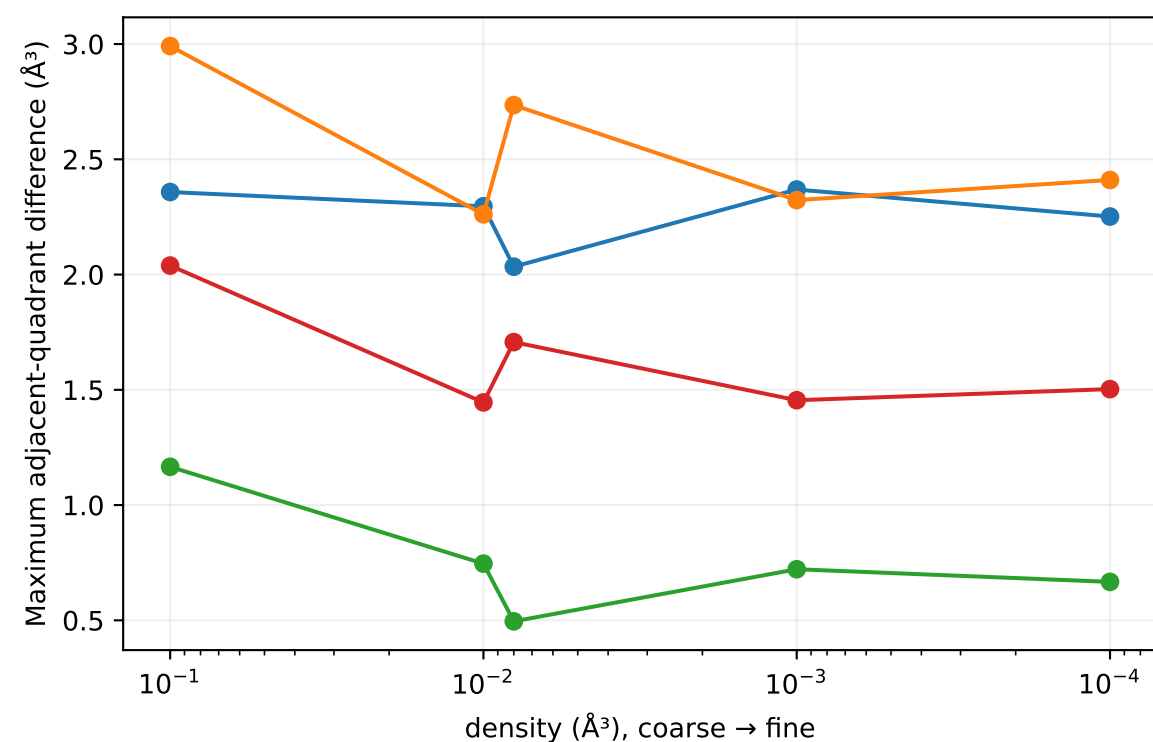
Frozen StericX convergence: odd-grid regional bias is retained
